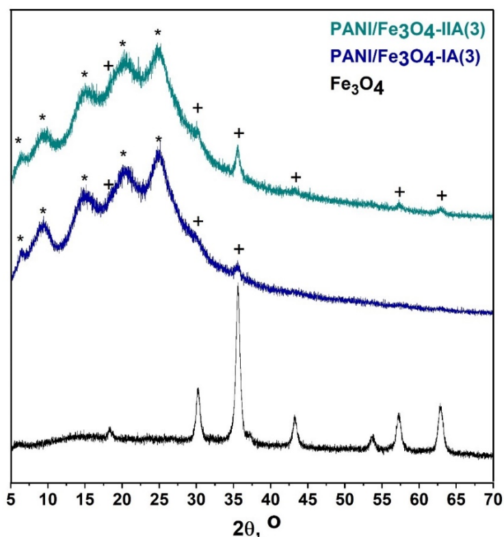
Slika 4.21. Difraktogrami prahova PANI/ \text{Fe}_3\text{O}_4 -IIA(3), PANI/ \text{Fe}_3\text{O}_4 -IA(3) i \text{Fe}_3\text{O}_4 .
